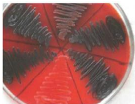
Figure 4: Modified Congo Red Agar method for detection of biofilm formation
