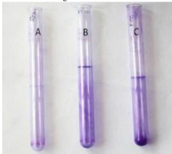
Figure 1: Tube method for detection of biofilm formation
