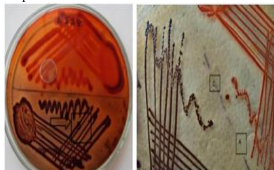
Figure 3: Congo red agar method for detection of biofilm formation
